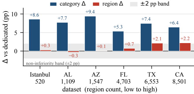
Fig. 4. Signed gains of the joint model over the dedicated single-task models, ordered by region count. The category gain (macro-F1) is positive at every dataset; the region gain (Acc@10) rises with region count across the five U.S. states and is also positive at Istanbul. The two metrics are on different scales; the \pm 2 -point band applies to region.
