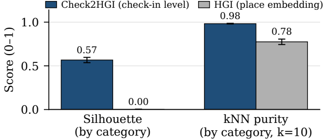
Fig. 3. Class separability of the representations, grouping each vector by its ground-truth category label (cosine silhouette; leave-one-out nearest-neighbor (kNN) purity, k=10 ), averaged over the five U.S. states. The check-in-level representation separates the seven categories; the place embedding does not.
